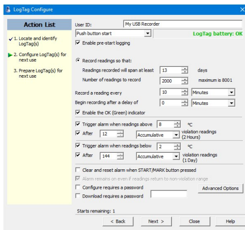
Figure 1: USRIC-8(M) Standard Configuration Options
